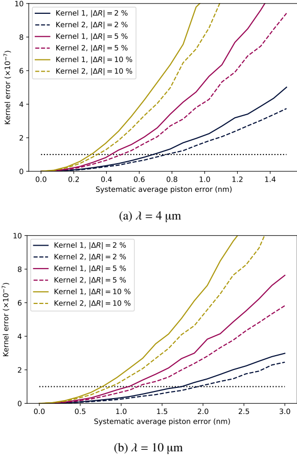
Fig. 7: Error in the kernel, plotted against systematic piston error in nanometers for a variety of optical beam combiner errors. The dotted line at 1 \times 10^{-7} represents the point where the kernel should be sensitive enough to detect an Earth-like planet around a solar type star.
