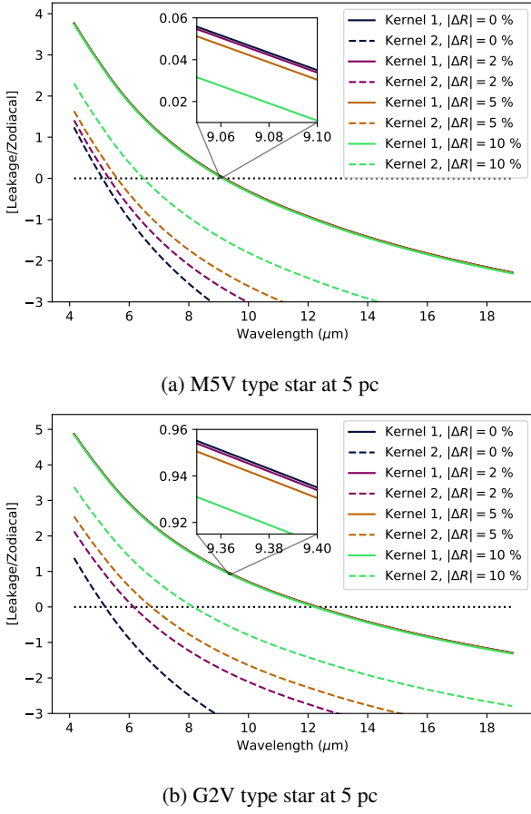
Fig. 5: Base-10 logarithm of the ratio of the stellar leakage to zodiacal light against wavelength for two different stars and varying amounts of beam combiner optical error. The black dashed line divides the upper region where the combiner is dominated by stellar leakage, and the lower region where the instrument is zodiacal limited. The inset highlights the proximity of the different optical error lines for kernel 1.
