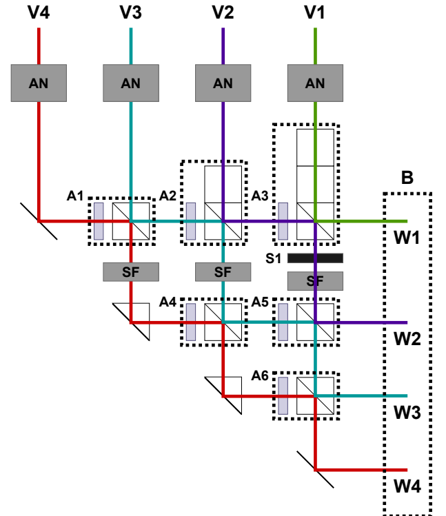
Fig. 13: Schematic of an X-array beam combiner based on the design of Guyon et al. (2013). The design is the same as in Figure 1, except with four inputs and outputs, and the optical parameters found in Table 3.
