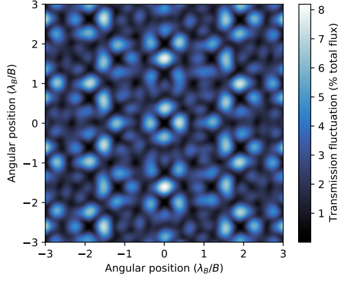
(a) Kernel 1
