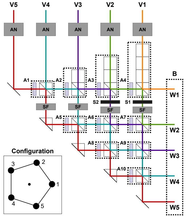
Fig. 1: Schematic of a Kernel-5 beam combiner, based on the design of Guyon et al. (2013). Inputs \mathbf{V}_1 through \mathbf{V}_5 pass through five adaptive nuller units (AN), a series of ten beam splitter modules ( \mathbf{A}_1 through \mathbf{A}_{10} ) consisting of a beam splitter and phase shifting plate on one input, and four spatial filters (SF). The five outputs consist of one bright output \mathbf{W}_1 and four nulled outputs \mathbf{W}_2 through \mathbf{W}_4 . Two shutters (S) can be used in case of a telescope failure (see Section 4). The inset shows the telescope configuration and their corresponding inputs.
