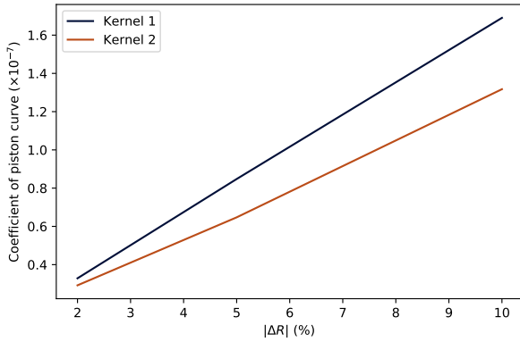
Fig. 8: Relationship between the quadratic coefficients of Figure 7b and their associated error in the beam combiner |\Delta R| .
