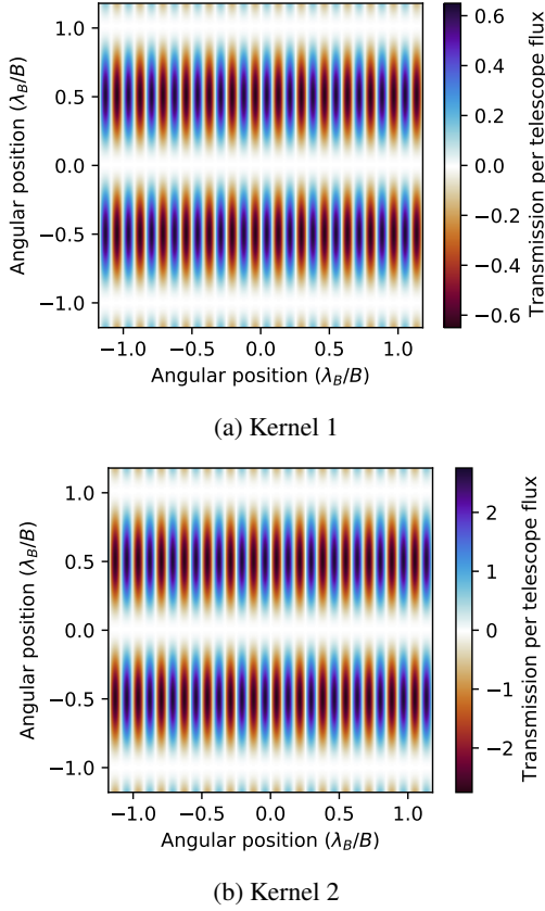
Fig. 11: Kernel maps of the ‘damaged’ Kernel-5 beam combiner with four telescope inputs. It is important to note the different scaling in the colour maps; this is due to a combination of the beam combiner architecture, along with the geometry of the array.
