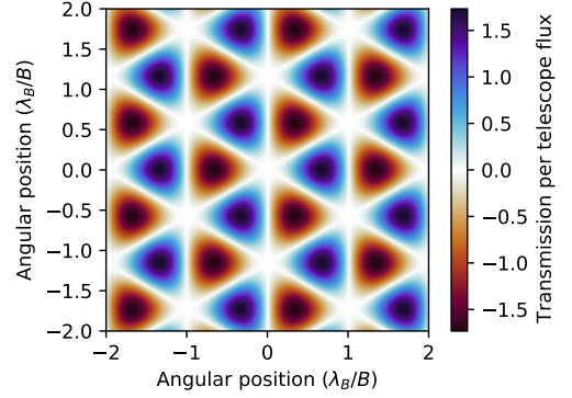
Fig. 15: Kernel map of the ‘damaged’ X-array type beam combiner with three telescope inputs.
